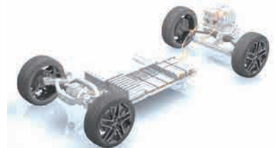
Electric drive parts that can potentially be converted to die casting
